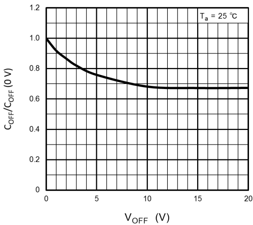
Fig. 12.11 COFF/COFF(0 V)-VOFF
